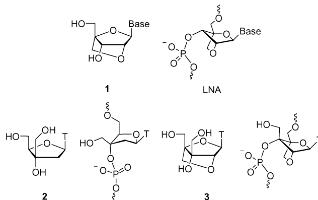
Figure 1. The general LNA nucleoside monomer 1 and the N -type conformation of LNA, 3'-C-(Hydroxymethyl)thymidine 2 and the 3'-C-hydroxymethyl LNA thymidine monomer 3 as well as their incorporation in nucleic acids as S -type and N -type mimics, respectively. T = thymine-1-yl.
