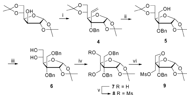
Scheme 1. Reagents and conditions: i. ref. [13] , 68%; ii. a) RuCl 3 ·xH 2 O, NaIO 4 , H 2 O, EtOAc, CH 3 CN; b) NaBH 4 , H 2 O, THF; c) NaIO 4 ; d) NaBH 4 , 74%; iii. a) BnBr, NaH, DMF; b) 80% aq. CH 3 COOH, 74%; iv. a) NaIO 4 , H 2 O, THF; b) HCHO, NaOH, 93%; v. MsCl, pyridine, quantitative; vi. NaOBz, DMF, 82%.
