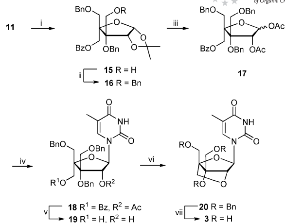
Scheme 3. Reagents and conditions: i. a) BzCl, pyridine; b) \text{RuCl}_3 \cdot x\text{H}_2\text{O} , \text{NaIO}_4 , \text{H}_2\text{O} , EtOAc, \text{CH}_3\text{CN} ; c) \text{NaBH}_4 , \text{H}_2\text{O} , THF; d) \text{NaIO}_4 ; e) \text{NaBH}_4 ; 71%; ii. BnBr, NaH, DMF, 75%; iii. a) 80% aq. \text{CH}_3\text{COOH} ; b) \text{Ac}_2\text{O} , pyridine, 91%; iv. Thymine, BSA, TMS-triflate, \text{CH}_3\text{CN} , 93%; v. \text{NaOCH}_3 , MeOH, 86%; vi. a) MsCl, \text{CH}_2\text{Cl}_2 , pyridine; b) NaH, 1,4-dioxane, 72%; vii. \text{H}_2 , \text{Pd}(\text{OH})_2/\text{C} , EtOH, quantitative.
