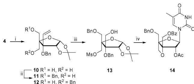
Scheme 2. Reagents and conditions: i. a) \text{H}_5\text{IO}_6 , EtOAc; b) \text{HCHO} , NaOH, \text{NaBH}_4 , 94%; ii. NaH, BnBr, DMF, 60% 11 and 28% 12 ; iii. a) MsCl, Pyridine; b) \text{RuCl}_3 \cdot x\text{H}_2\text{O} , \text{NaIO}_4 , \text{H}_2\text{O} , EtOAc, \text{CH}_3\text{CN} ; c) \text{NaBH}_4 , \text{H}_2\text{O} , THF; d) \text{NaIO}_4 ; e) \text{NaBH}_4 ; 54%; iv. a) BzCl, pyridine; b) 80% aq. \text{CH}_3\text{COOH} ; c) \text{Ac}_2\text{O} , pyridine; d) thymine, BSA, TMS-triflate, \text{CH}_3\text{CN} , 20%.
